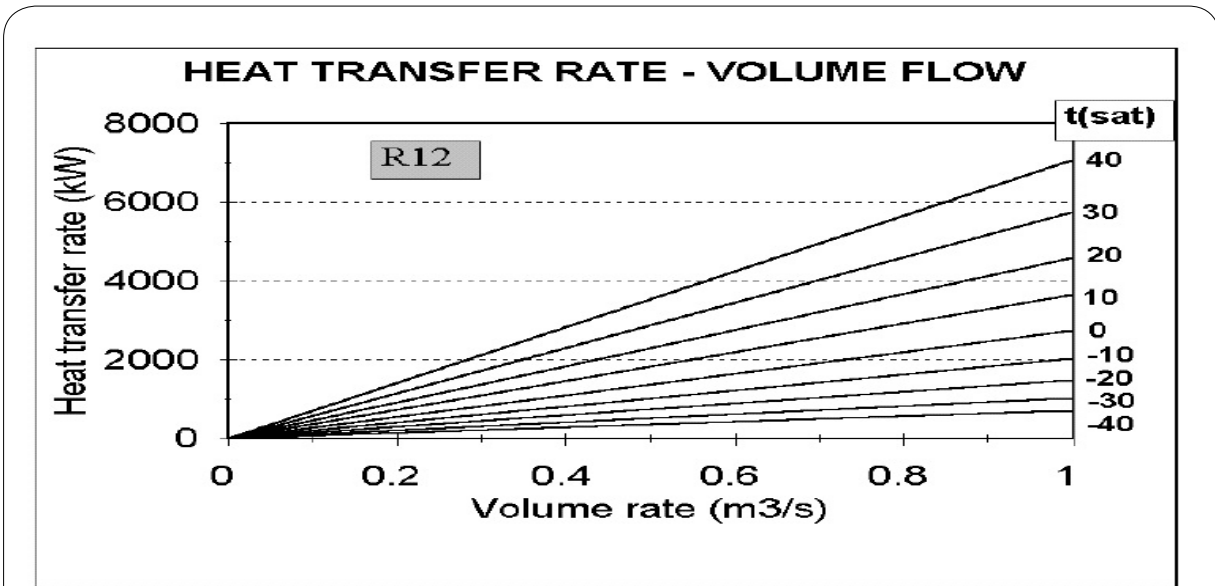
Figure 5: Heat transfer rate versus volume rate.
