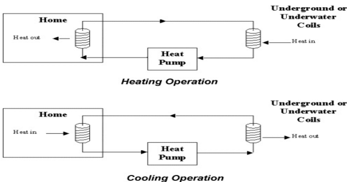
Figure 10: Heating and cooling operations.
